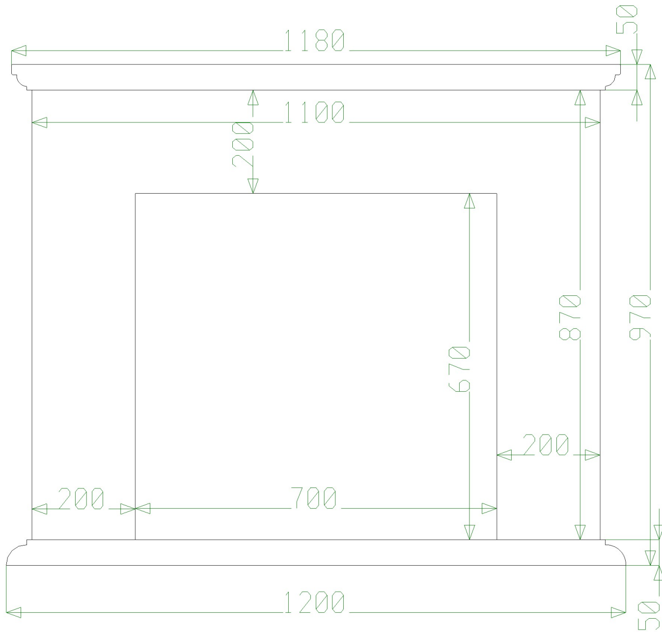
Front View
