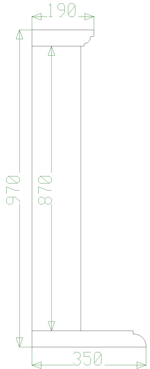
Side View
